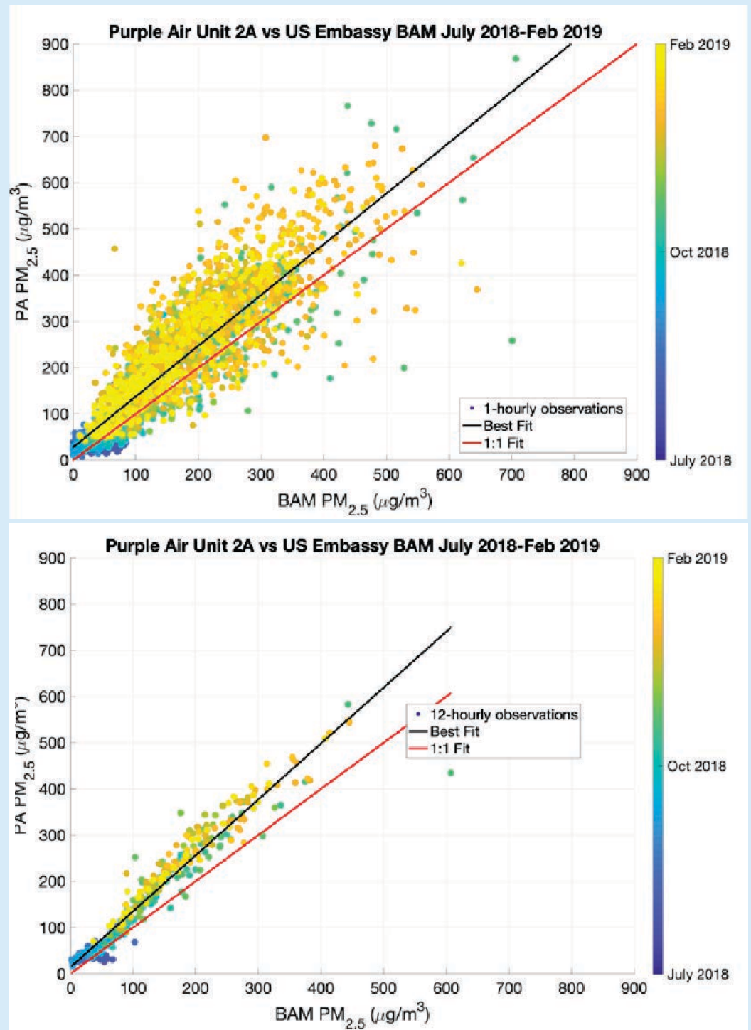
Figure 8. Hourly (upper row) and 12-hourly (bottom) average concentrations for PurpleAir sensor vs U.S. Embassy BAM reference monitor, July 2018 - February 2019.
